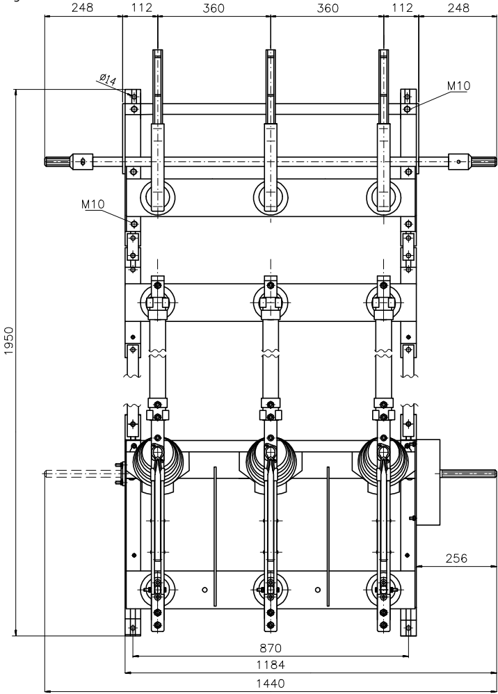
NALF 36 + EB on opening side
