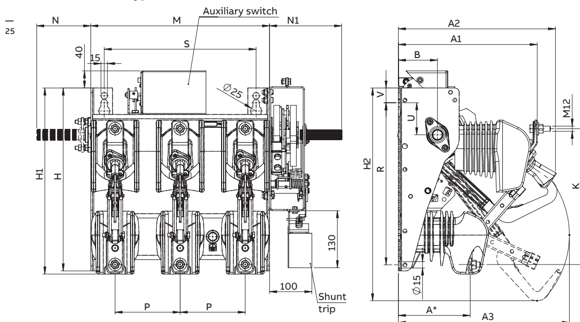
Switch-disconnector type NAL - H (12, 17.5 and 24 kV) with mechansim
