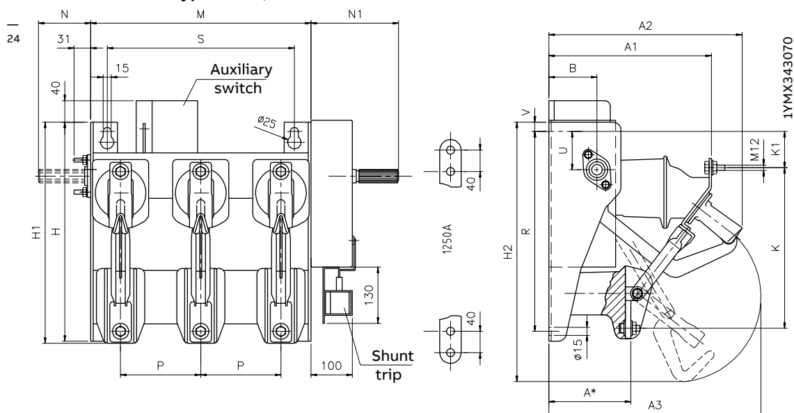
Switch-disconnector type NAL - H (12, 17.5 and 24 kV) with mechansim
