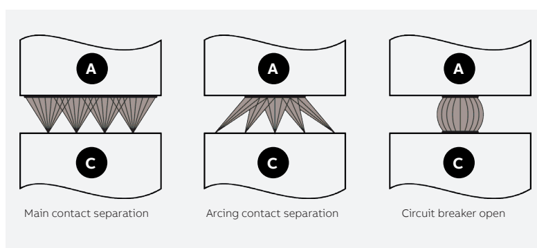
Diagram of transition from diffuse arc to constricted arc in a vacuum interrupter
