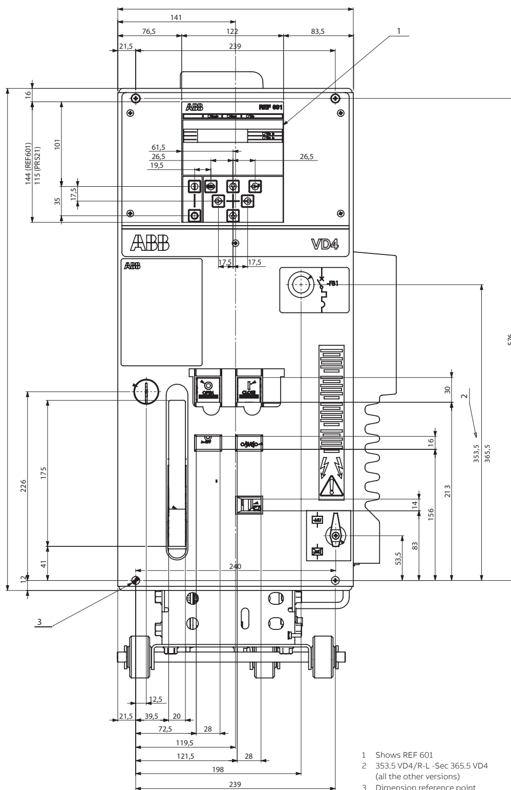
Detail of control front
