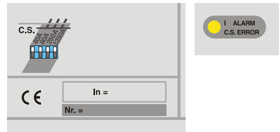
Selection of the primary current of the current sensors
