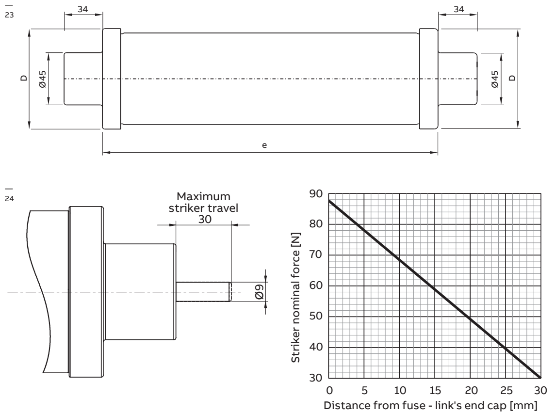
24 Fuse-link striker force and dimensions
