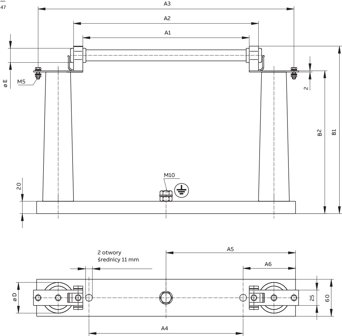
47 Dimensional drawings of fuse-bases type PBPM-20, PBPM-30
